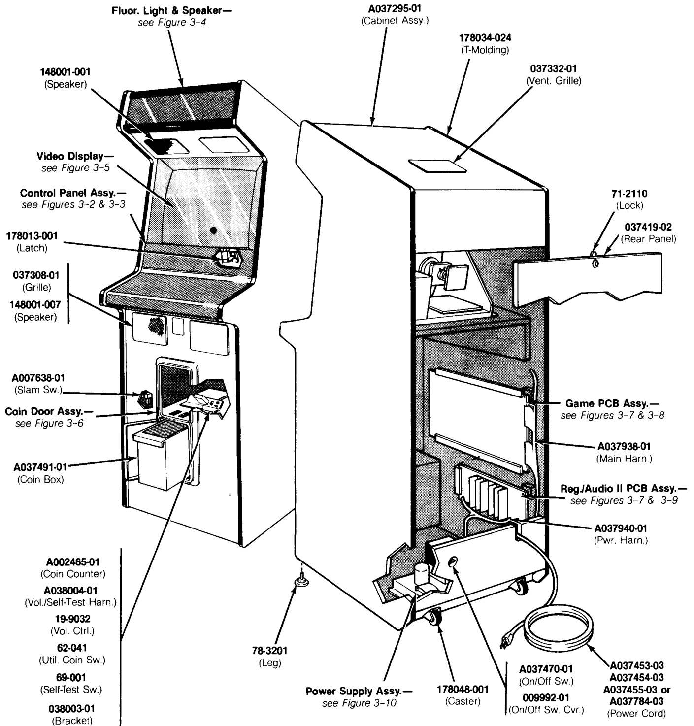
Figure 3-1 Upright Cabinet-Mounted Assemblies A037294-xx B
