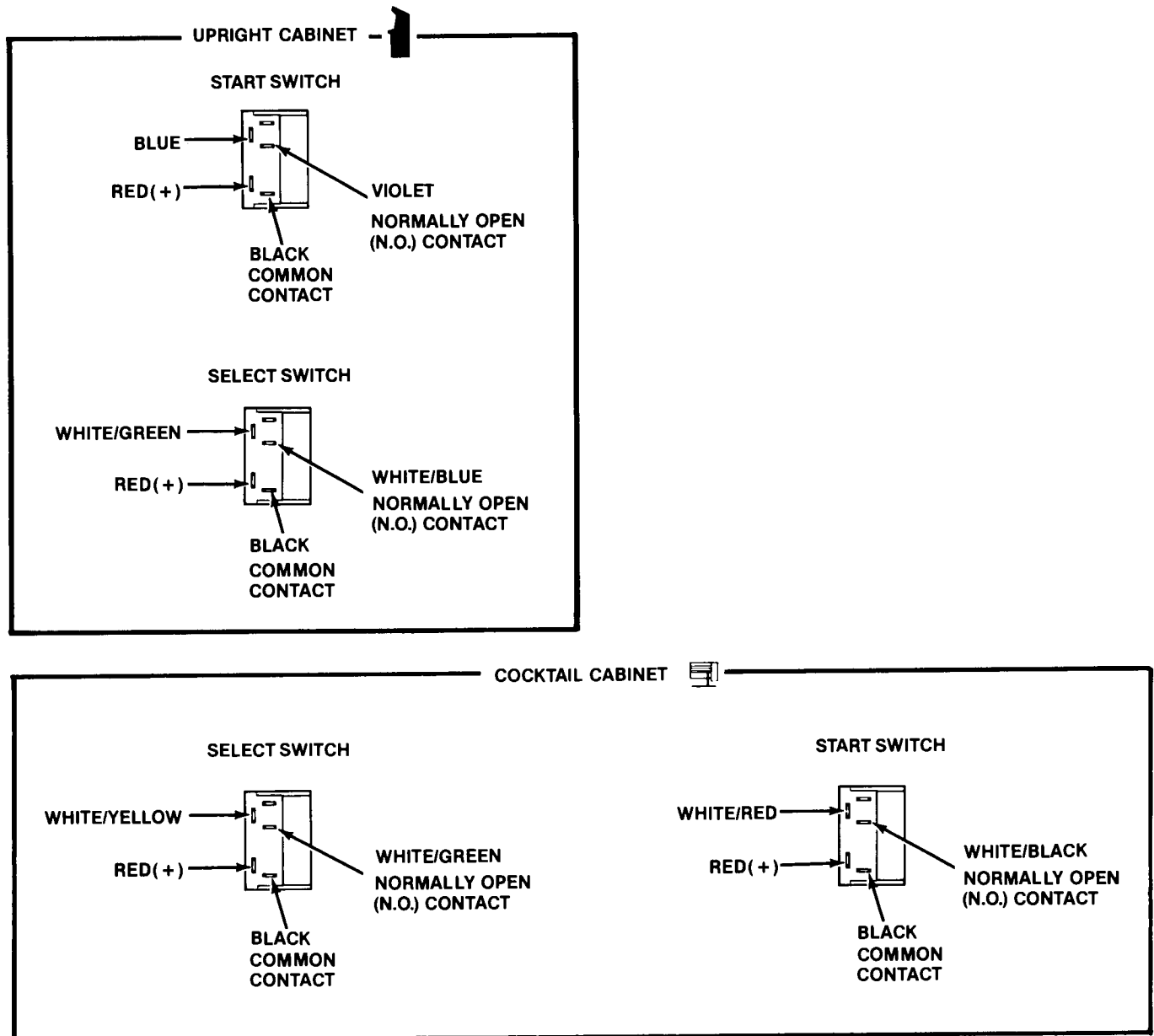
Figure 3-2 The Control Panel, continued
