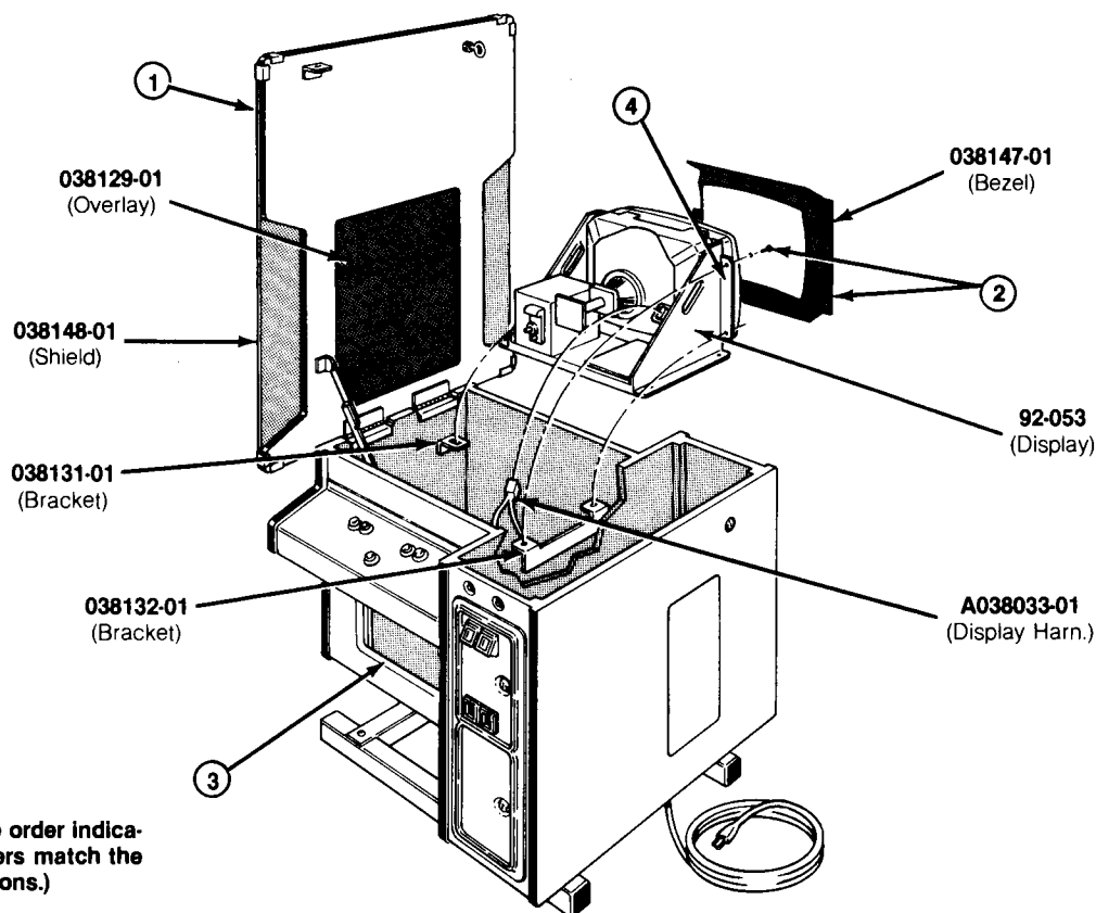
Figure 3-5 continued, Cocktail Video Display Removal VA037294-01 A and VA038100-01 A Parts List
