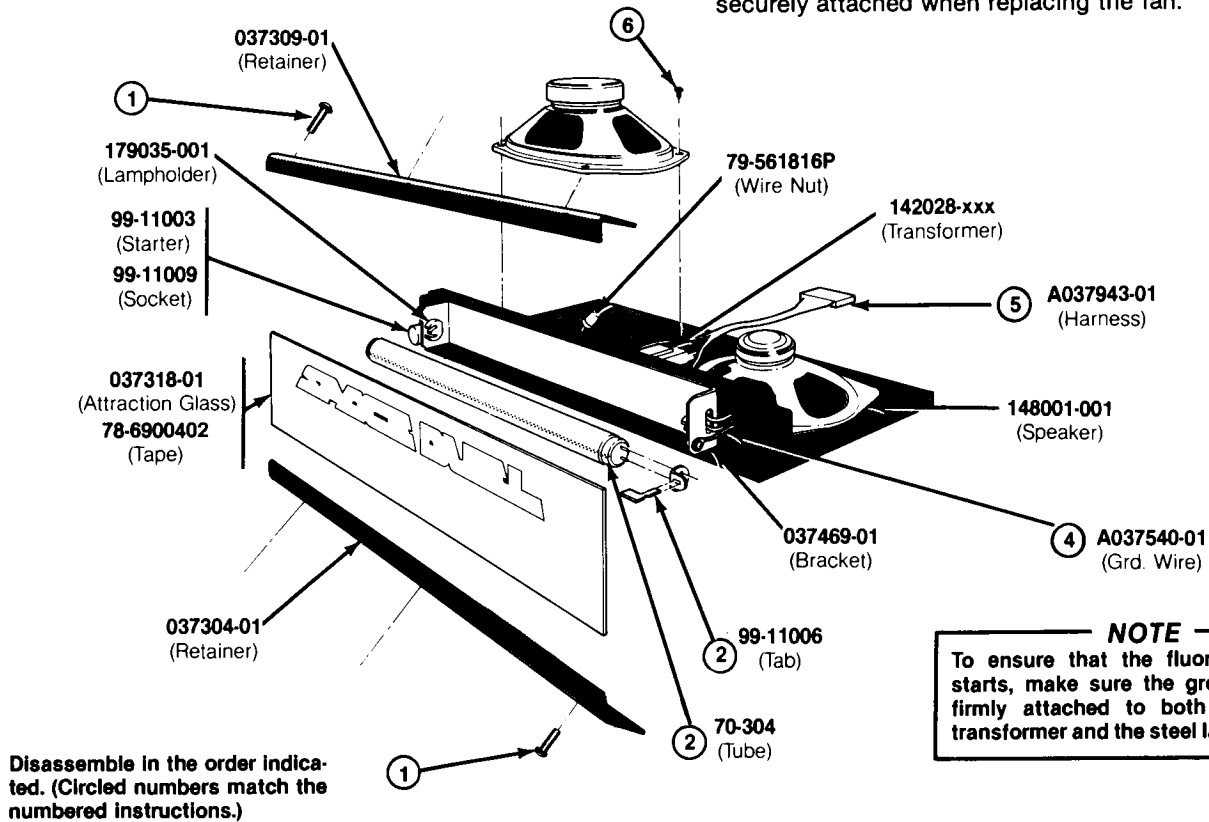
Figure 3-4 Speaker, Fluorescent Tube and Fan
